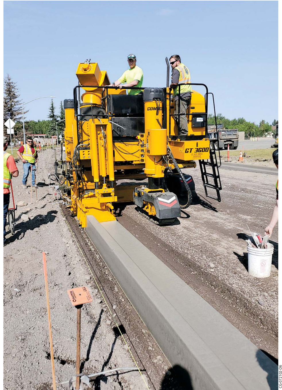
The exclusive, independent adjustable stainless steel troweling section seals and provides the superior GOMACO finish.
