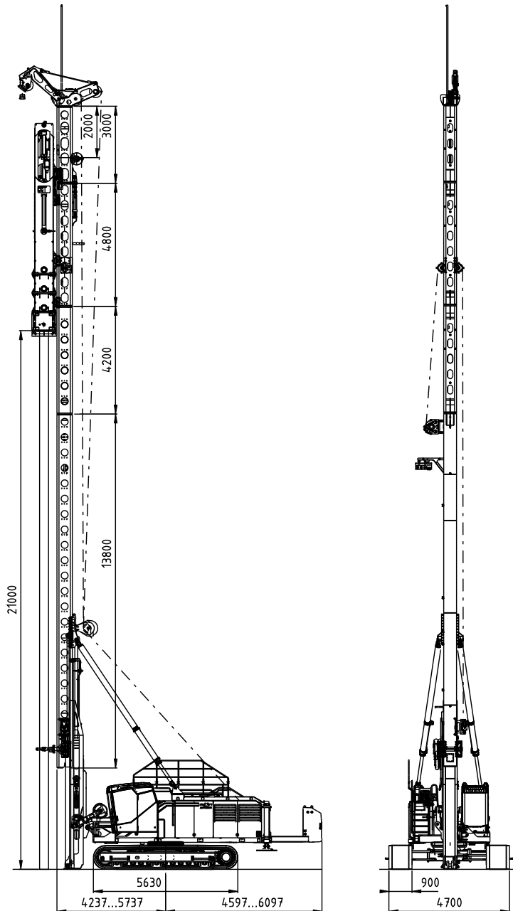
PMz6 with Junttan Hydraulic Impact Hammer HHK5/7/9S
