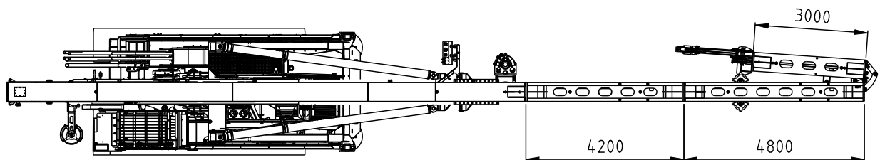
PMz6 transport dimensions with Junttan Hydraulic Impact Hammer HHK5/7/9S
