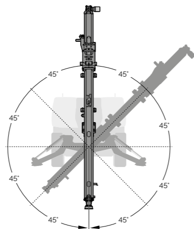
Alternative B: Re-pinning in steps of 45° enabling drilling in 360°
